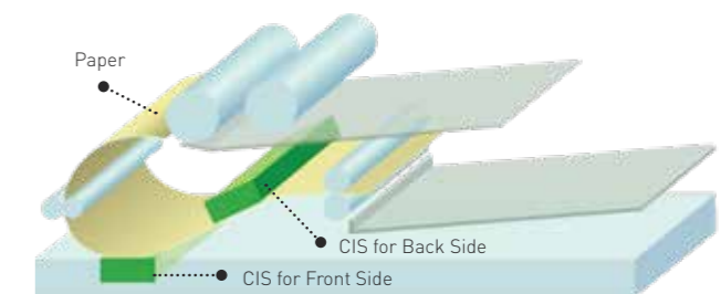
Diagram shows placement of both Contact Image Sensors (CIS) for enhanced scanning speed.
